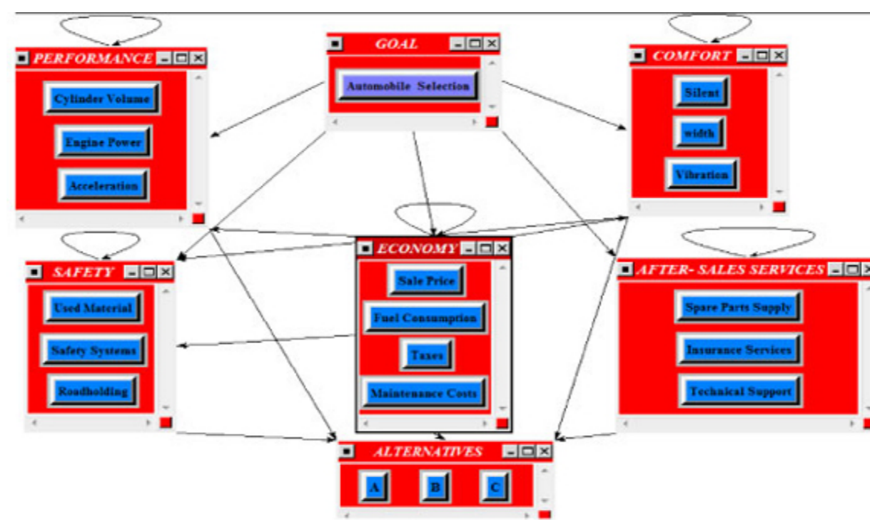
Figure 3: Screening of network structure formed for fuzzy ANP in Super Decisions 1.6 software package
